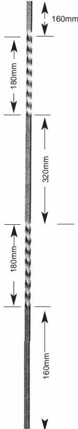
NB63-05 1000mm 12mm \varnothing NB63-06 1000mm 14mm \varnothing
