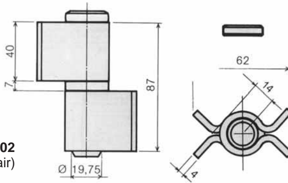
Fixed Pin
