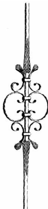
NB62-05 1000 x 225mm 14mm \varnothing
