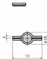
NB55-07 Loose Pin
