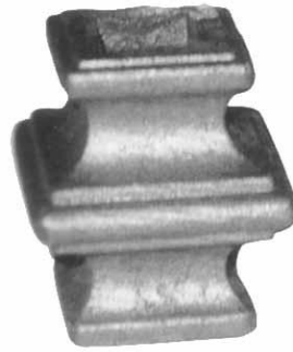
NB24-15 48 X 48 X 44 H MM 17 MM SQUARE HOLE
