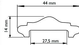
NB17-80 44 X 14 mm 3 mtrs Long
